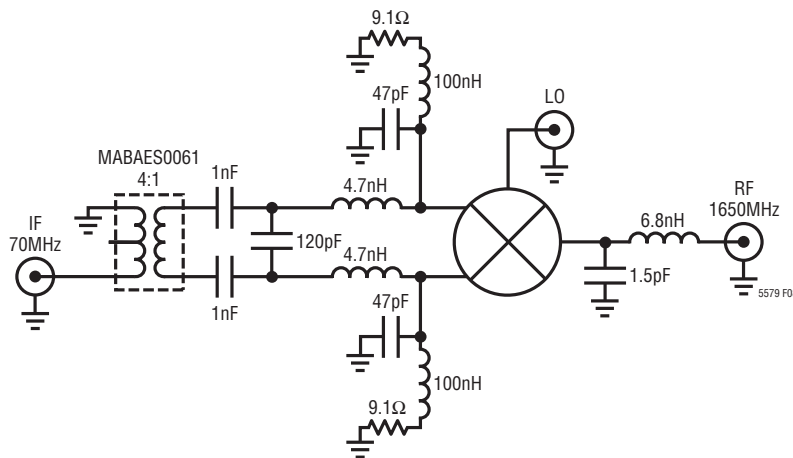
Figure 8. IF Input Tuned for 70MHz
